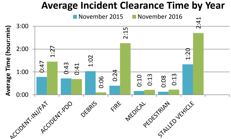
Figure 7: Average Incident Clearance time (2016 vs. 2015). Construction and tow events excluded for clarity.
